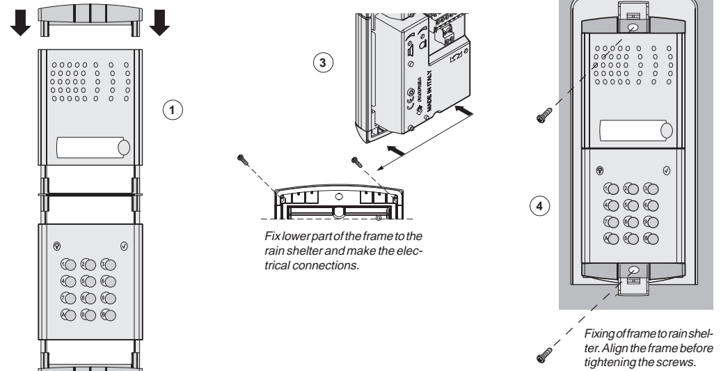
Mounting modules.
